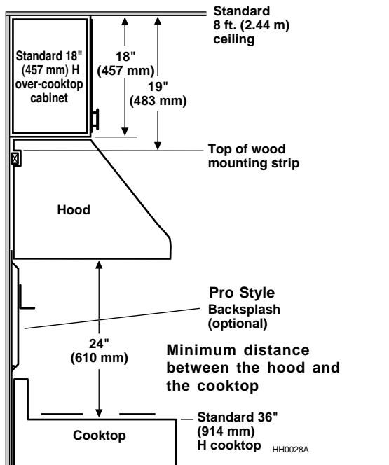
INSTALLATION WITH STANDARD 18" HIGH OVER-COOKTOP CABINET
